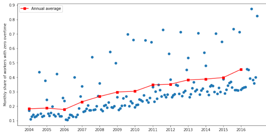
(b) Share of worker with zero overtime
